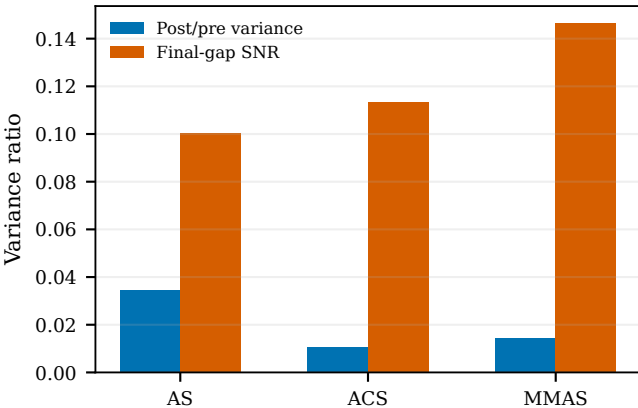
2-opt compression and final signal
