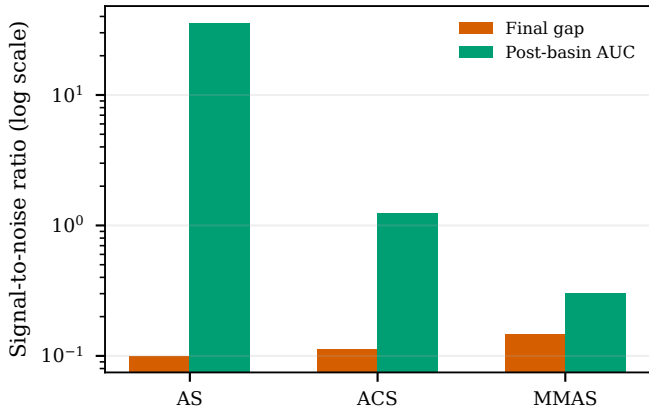
Alternative learning signals
